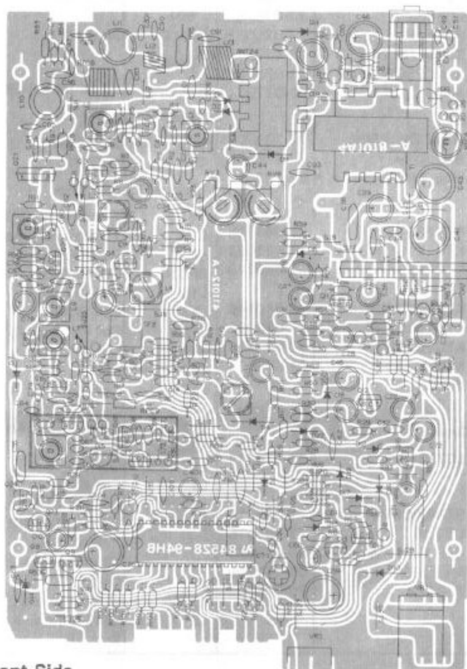
Component Side.
